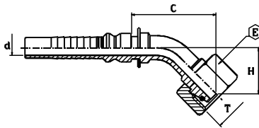
METRIC FEMALE 24° FLARE HEAVY 45° ELBOW
