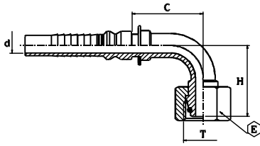
METRIC FEMALE 24° FLARE HEAVY 90° ELBOW
